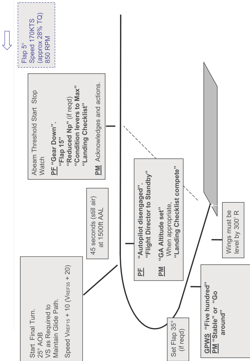
Figure 12.1 Visual Circuit
